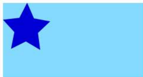
kCAGravityTopLeft
